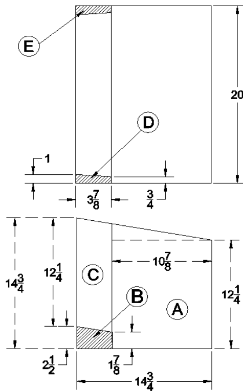
Firebox Volume Sketch
